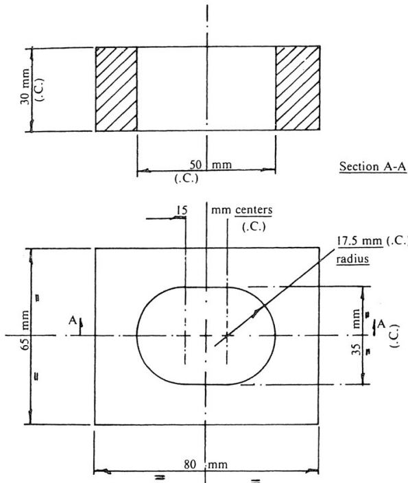
(C.C.) Dimensions critical \pm 0.5 mm
