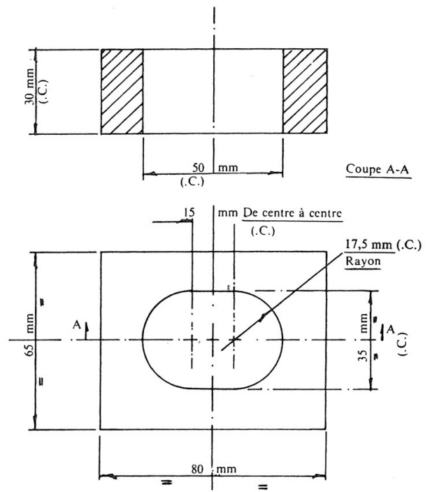
(C.C.) Dimensions limites \pm 0.5 mm
